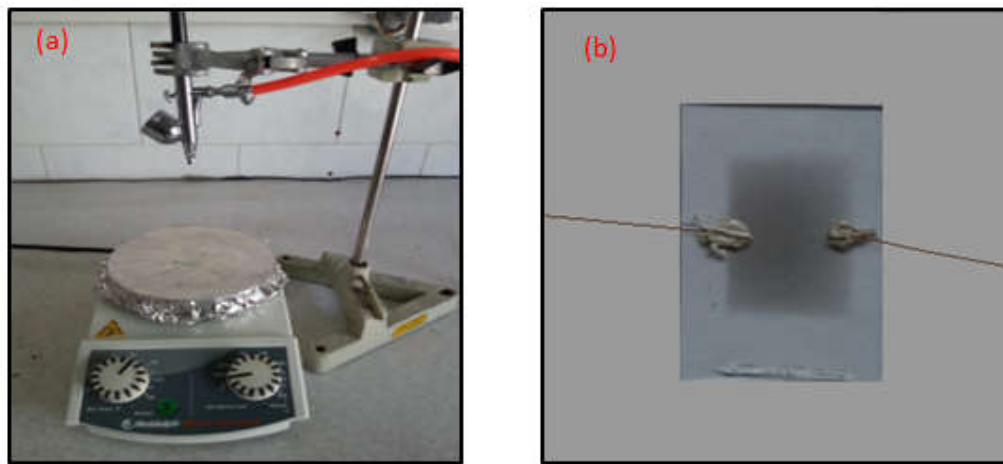
Figure 5. (color online) (a) Spray setup. (b) Graphene on the substrate.
