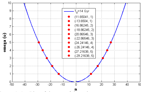
Figure 1. (co Plot of the age of the universe.
