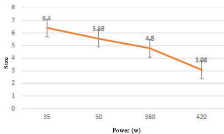
Figure 4. (color online) Ultrasonic relation to the size of the graphene sheets.
