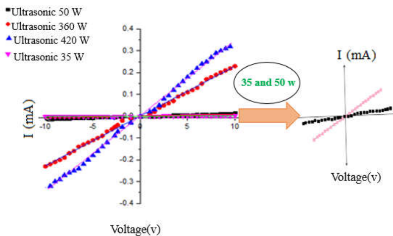
Figure 6. (color online) I-V Behavior of four samples
