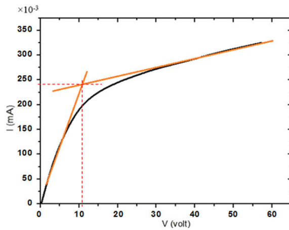
Figure 6. (color online) Characteristic I- V curve for typical argon and the way of drawing two tangent lines and the emerging junction point of coordinate (I, V).
