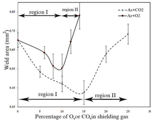
Figure 2. Weld area versus CO 2 or O 2 concentration in shielding gas.
