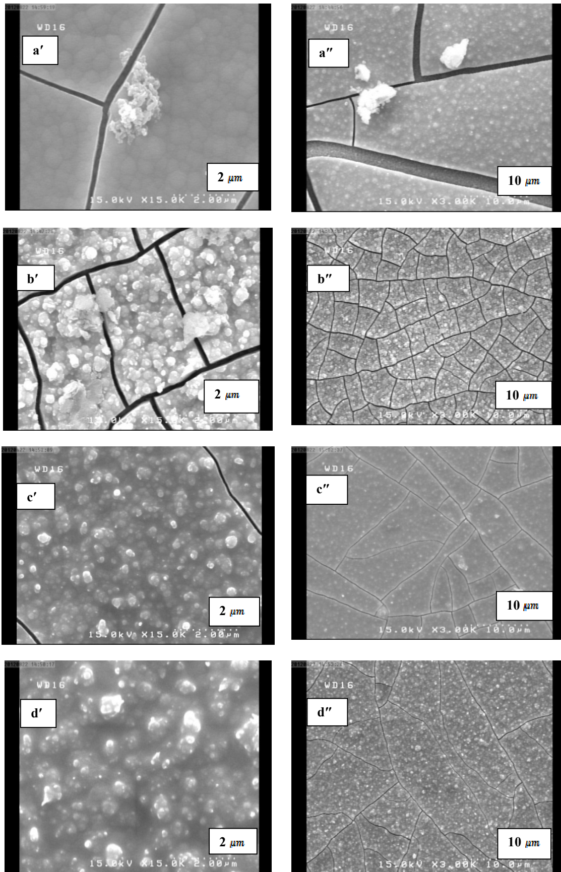
Figure. 1. SEM image of \text{WO}_3 films annealed at 60°C (a', a''), 100°C (b', b''), 250°C (c', c''), and 400°C (d', d'').
