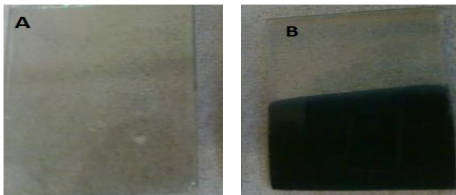
Figure 7. Transmittance change of WO 3 film annealed at 60 °C in a halfcell, (a) bleached state, (b) colored state.
