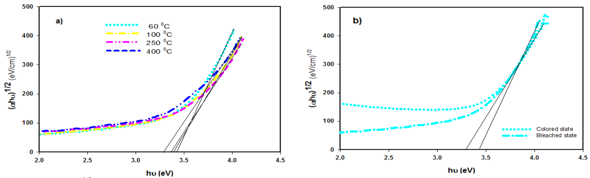
Figure 4. Plot (\alpha h\nu)^{1/2} vs. h\nu for WO 3 films annealed at (a) different temperatures in bleached state, (b) 60°C in colored and bleached states.
