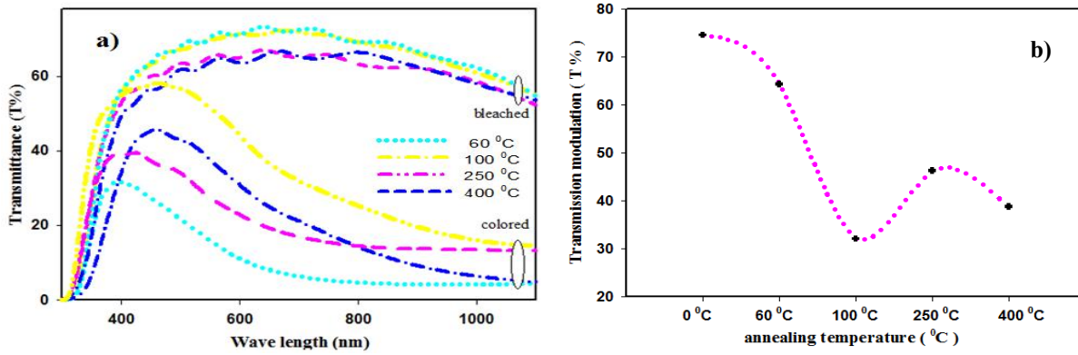
Figure 2. (a) Optical transmittance spectra of WO 3 thin films annealed at different temperatures in colored and bleached states within 300 \leq \lambda \leq 1100 nm range, (b) transmission modulation as a function of annealing temperature, as calculated from data in figure 3a.
