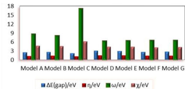
Figure 7. Plots of energy gap ( E_{gap} ), global hardness ( \eta ), electrophilicity index ( \omega ), and electronegativity ( \chi ) of (A–G) models (figure 1).
