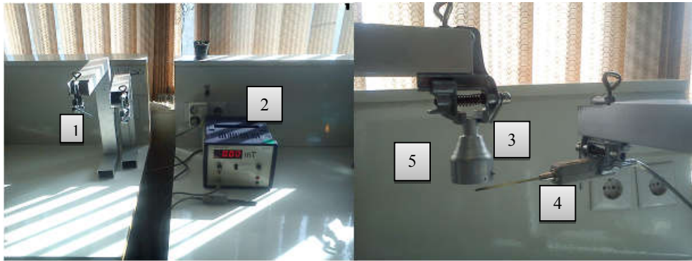
Figure 9. (color online) Measurement equipment (1) Aluminum stands, (2) phvwe teslameter device with a probe, (3) aluminum hook, (4) measurement probe, and (5) magnet aluminum fixture.
