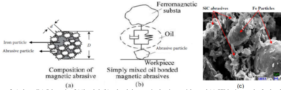
Figure 3. (color online) Schematic of (a) bonded, (b) unbonded magnetic abrasive particles, and (c) SEM micrograph of unbonded SiC abrasives (800 mesh).
