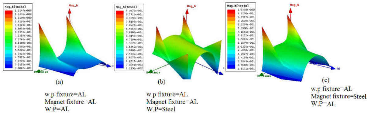
Figure 23. (color online) Magnetic flux density plot in 2 mm distance from the magnet surface.
