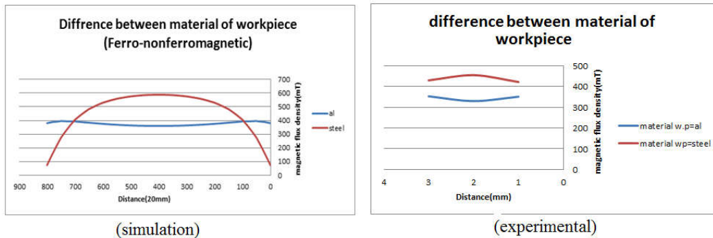
Figure 21. (color online) Simulation and measurement of the effect of work piece material on the magnetic flux density.
