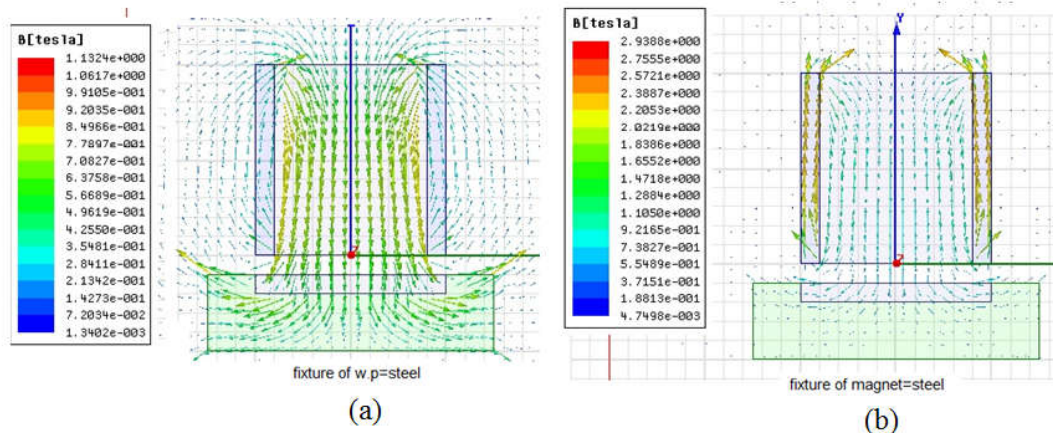
Figure 26. (color online) Establishment of the closed ring, (a) ferromagnetic work piece fixture, and (b) ferromagnetic magnet fixture.
