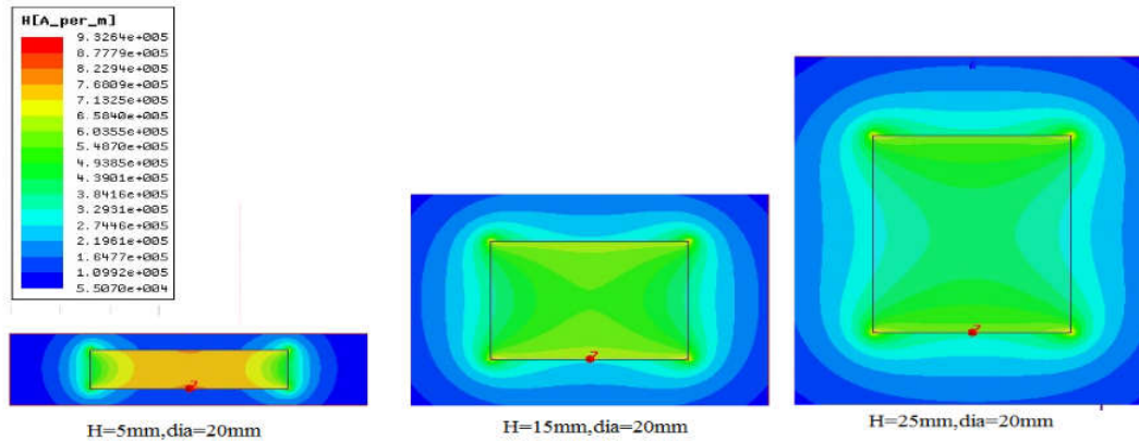
Figure 7. (color online) Magnetic field strength in different heights (dia, 20mm).
