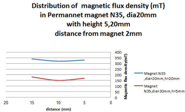
Figure 11. (color online) Magnetic flux distribution (militesla) in a magnet of 20 mm height and different heights in a 2 mm distance from the surface (measured).
