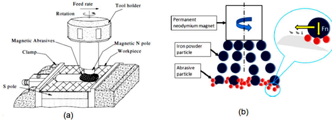
Figure 1. (color online) Magnetic abrasive finishing with the permanent magnet and the magnetic abrasive powder.
