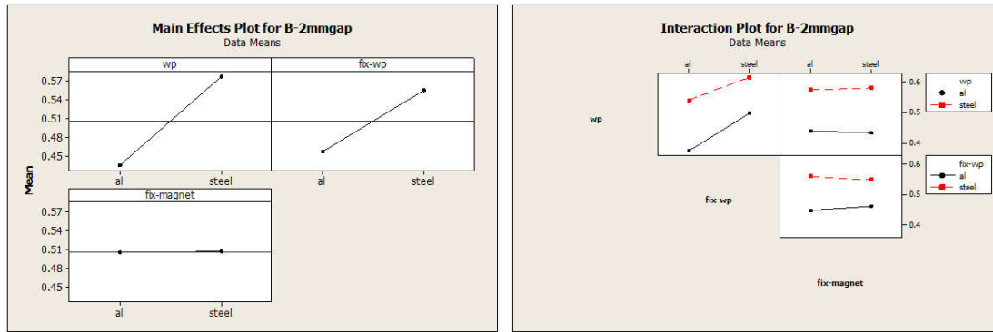
Figure 19. (color online) Main effect plot and the interaction plot for magnetic flux density (gap=2mm).
