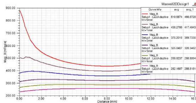
Figure 17. (color online) Magnetic field intensity distribution in different distances from the magnet.
