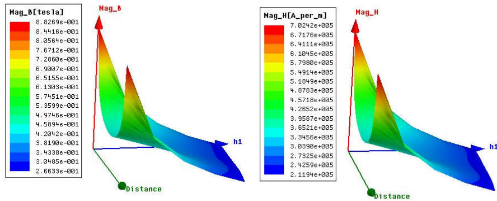
Figure 16. (color online) Magnetic flux density and field strength in a 16×20 mm magnet in different distances from the magnet.
