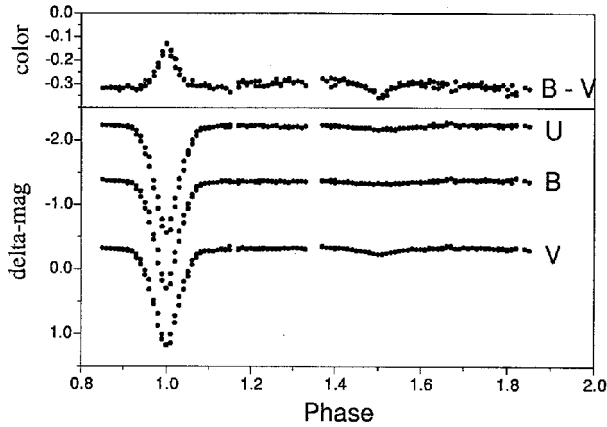
Figure 1. The light curves or RZ Cas for the U, B, and V filters.
