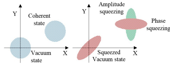
Figure 1. Vacuum state, coherent state, and squeezed states of light.
