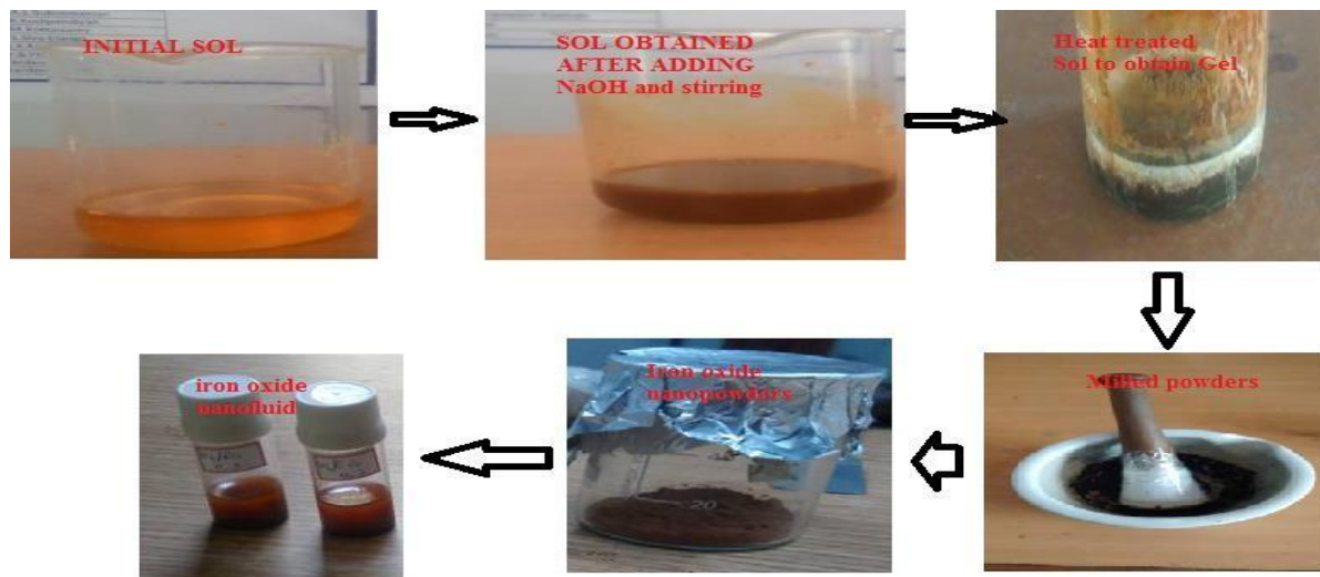
Figure 1. Synthesis of iron oxide – Ethylene Glycol nanofluid by our two step method.
