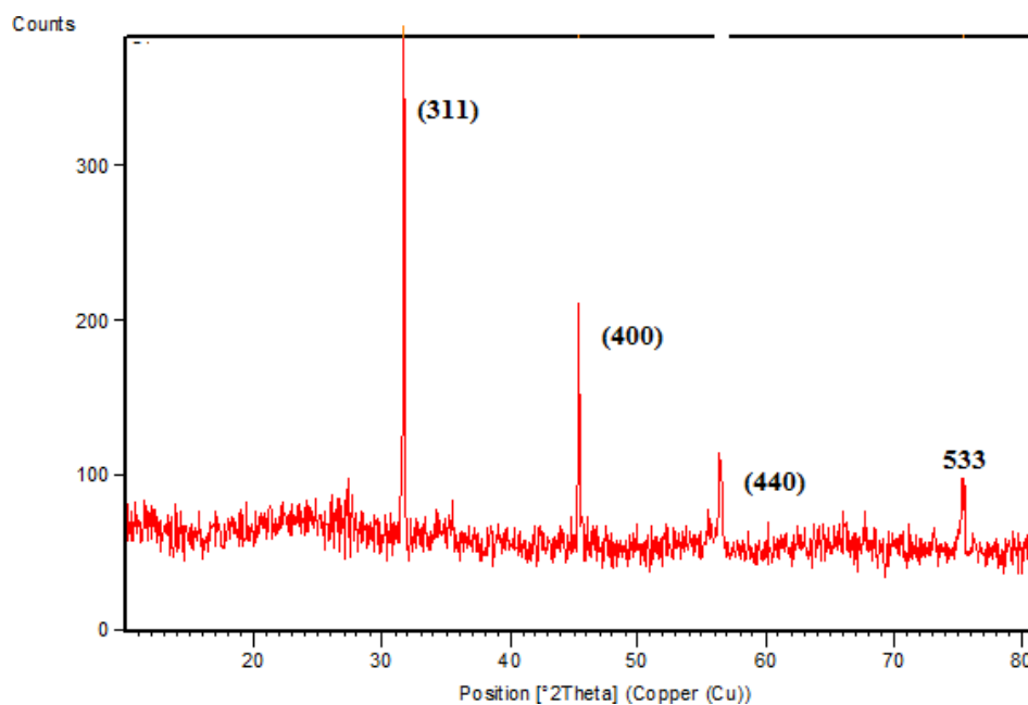
Figure 2. XRD pattern of the prepared iron oxide nanopowders.
