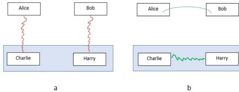
Figure 1: Entanglement Swapping. First in Fig. (a) There are 2 entangled pairs, one between Alice and Charlie, and the other one between Bob and Harry. There is no entanglement between Alice and Bob. However in Fig (b), the measurement on Charlie and Harry's qubits project the entanglement between Alice and Bob.
