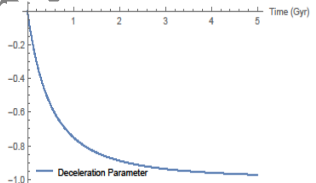
Figure 7: Variation of q vs. time t .
