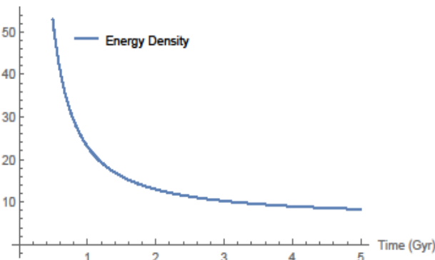
Figure 3: Variation of energy density \rho vs. time
