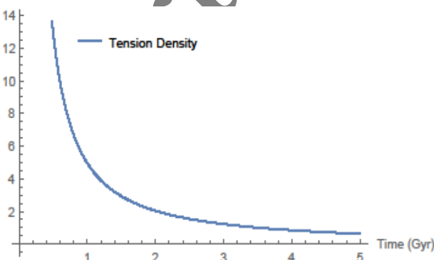
Figure 4: Variation of tension density \lambda vs. time
