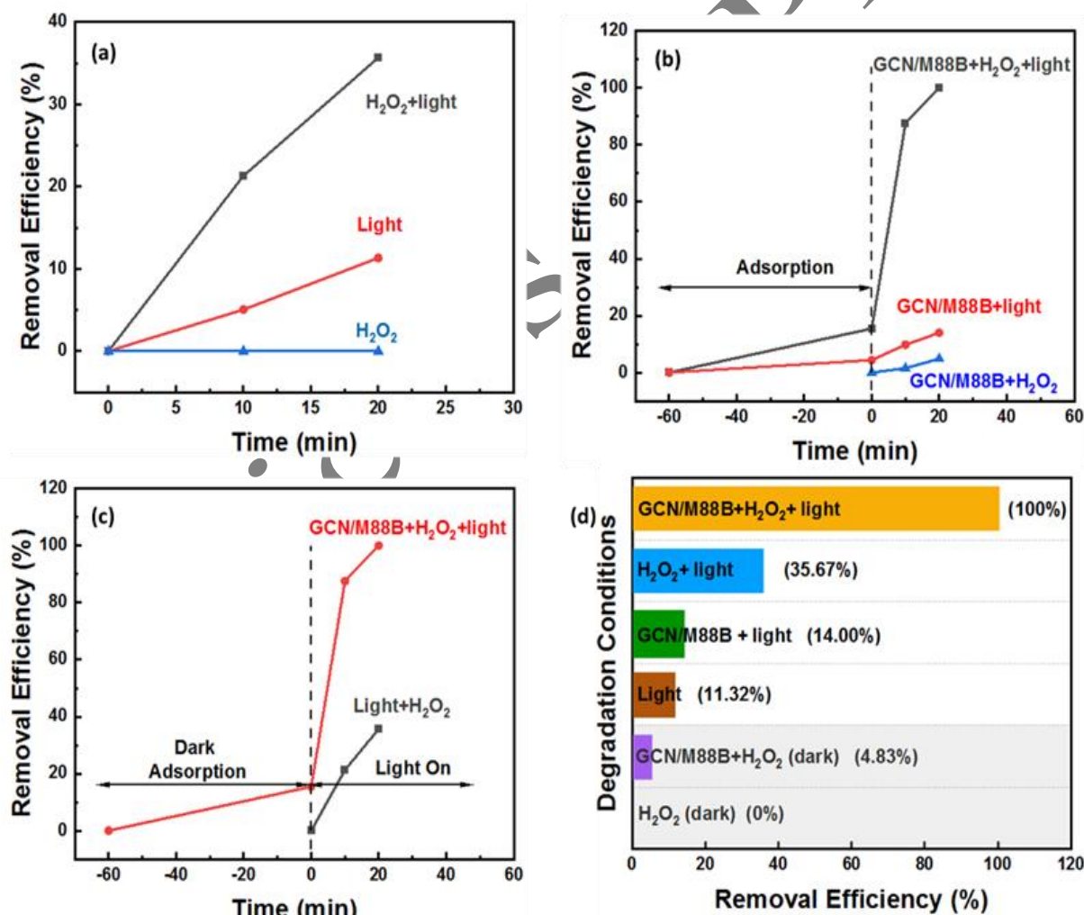
Figure 5. Removal efficiency of MB in the presence of; (a) Light+H 2 O 2 , Light, and H 2 O 2 (in 20 min), (b) g\text{-C}_3\text{N}_4/\text{MIL-88B(Fe)}+\text{H}_2\text{O}_2+\text{Light} , g\text{-C}_3\text{N}_4/\text{MIL-88B(Fe)}+\text{Light} , and g\text{-C}_3\text{N}_4/\text{MIL-88B(Fe)}+\text{H}_2\text{O}_2 (in 20 min), (c) g\text{-C}_3\text{N}_4/\text{MIL-88B(Fe)}+\text{H}_2\text{O}_2+\text{Light} , light+ H 2 O 2 (without nanocomposite). (d) Removal efficiencies vs. various degradation reaction conditions in 20 min (a summary of plots, presented in former panels). In all experiments the concentration of MB was 5 mg/L, the amount of H 2 O 2 was 15 \mu\text{L} , and the amount of photocatalyst was 10 mg. Also, the applied light source was in the range of UV-Vis.
