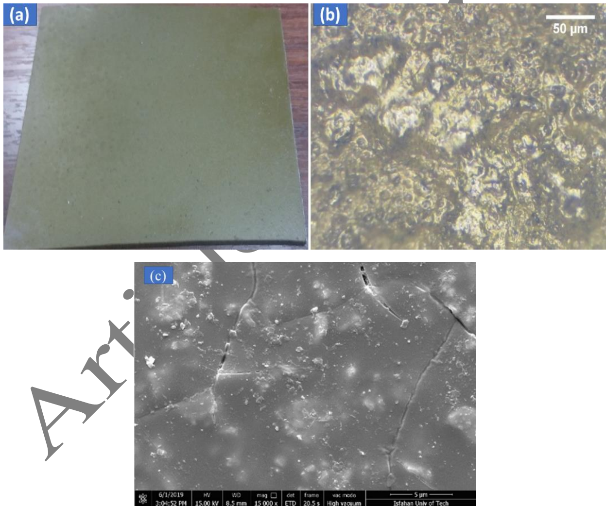
Fig. 2. (a) A digital photograph and (b) an optical micrograph of the surface of YIG paint at room temperature. and (c) FE-SEM micrograph of the paint after heating at 600 °C.
