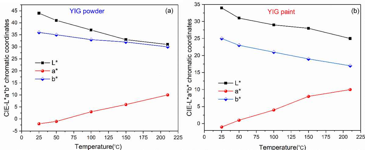
Fig. 6. Variation of Chromatic coordinates of (a) YIG powder and (b) YIG paint versus temperature.
