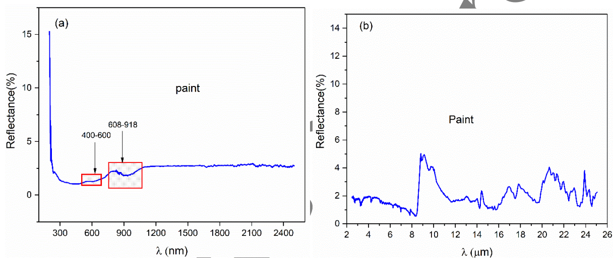
Fig. 4. Reflection spectrum of the yttrium iron garnet paint in (a) UV-Vis-near IR and (b) mid IR regions.
