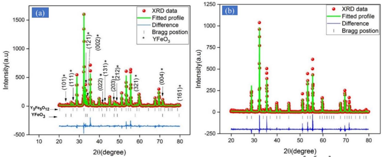
Fig. 1. XRD spectra of the garnet powder samples with their Rietveld analyses: (a) S-1200 and (b) S-1400.
