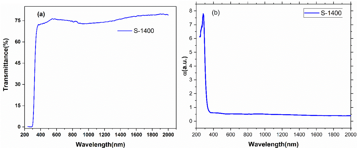
Fig. 3. (a) Transmission spectra and (b) absorption coefficient vs wavelength for (S-1400+ethylen glycol on glass).
