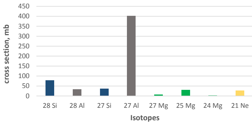
Fig.2. Cross section of the produced isotopes for the reaction between an incident neutron and ^{28}\text{Si} in E_n = 24.6 MeV
