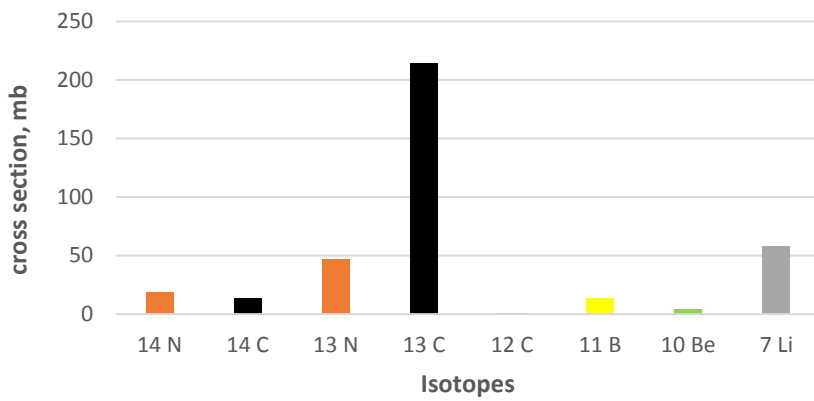
Fig.5. Cross section of the produced isotopes for the reaction between an incident neutron and ^{14}\text{N} in E_n = 24.6 MeV
