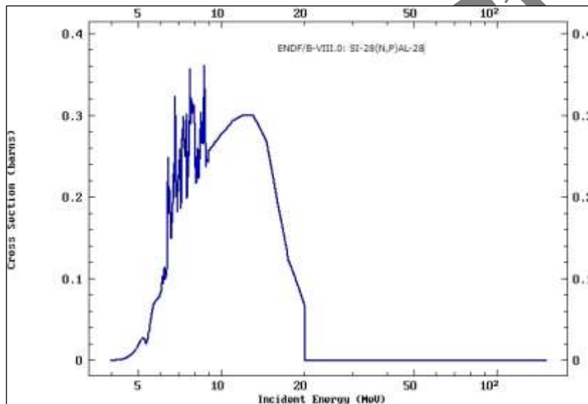
Fig. 8. Cross section of inelastic scattering for ^{28}\text{Si} (n, p) ^{28}\text{Al} within various energy ranges of neutron
