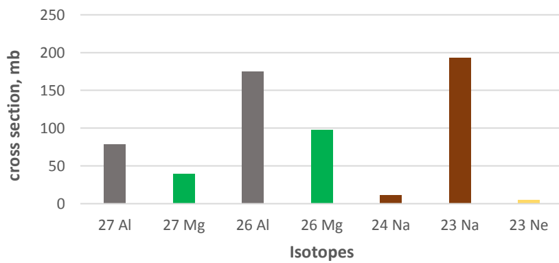
Fig.3. Cross section of the produced isotopes for the reaction between an incident neutron and ^{27}\text{Al} in E_n = 24.6 MeV
