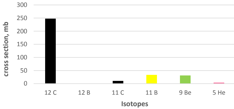
Fig.4. Cross section of the produced isotopes for the reaction between an incident neutron and ^{12}\text{C} in E_n = 24.6 MeV
