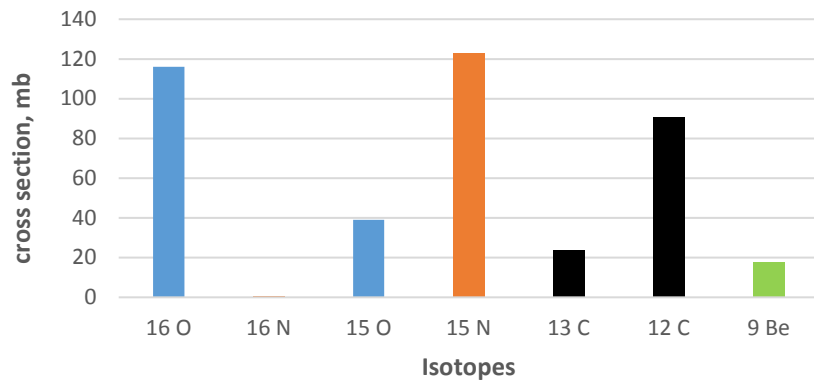
Fig.1. Cross section of the produced isotopes for the reaction between an incident neutron and ^{16}\text{O} in E_n = 24.6 MeV
