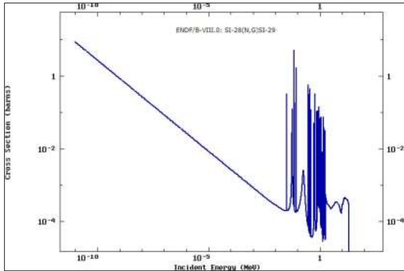
Fig. 7. Cross section of capturing reaction for ^{28}\text{Si} (n, \gamma) ^{29}\text{Si} within various energy ranges of neutron
