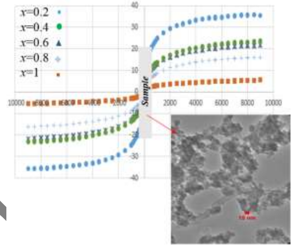
Fig. 4. The diagram of M-H samples, the TEM images of Co_{0.8}Zn_{0.2}Fe_2O_4 sample (at the right).
