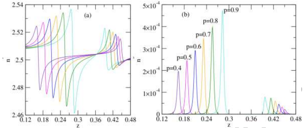
Figure 1. Passive composite with metal coated dielectric spherical Nano inclusions ( \epsilon_d'' = 0.0 ). Real part of the refractive index ( n' ) versus the dimensionless frequency ( z ) (a); imaginary part of the refractive index ( n'' ) versus z (b). Numerical values of composite parameters; fraction of inclusions in the composite f = 0.001
