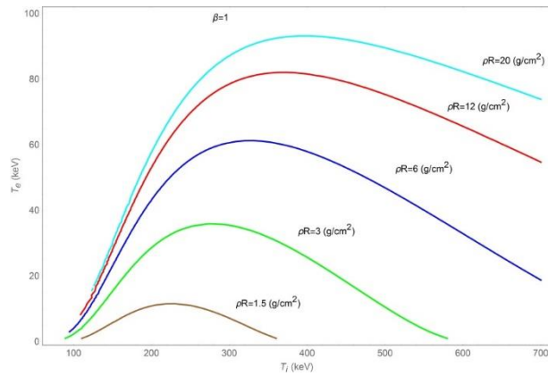
Figure 1. Variation of the confinement parameter, \rho R , with respect to ion and electron temperatures.
