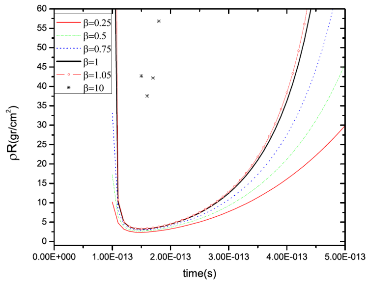
Figure 4. Investigating the temporal changes in the confinement parameter, ρR, in relation to fluctuations in temperature turbulence.
