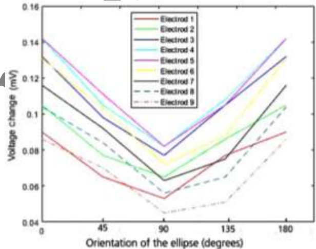
Figure 11 Voltage disturbance of each electrode as a function of the ellipse' orientation.
