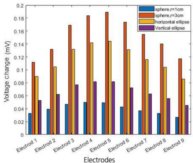
Figure 12 Compare voltage disturbance of each electrode for horizontal ellipse, vertical ellipse, spheres with radius 3 cm and 1 cm
