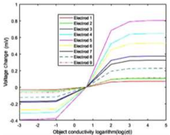
Figure 6 Voltage disturbance of each electrode as a function of the object conductivity logarithm.
