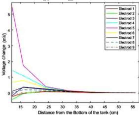
Figure 3 Voltage disturbance of each electrode as a function of the object distance.
