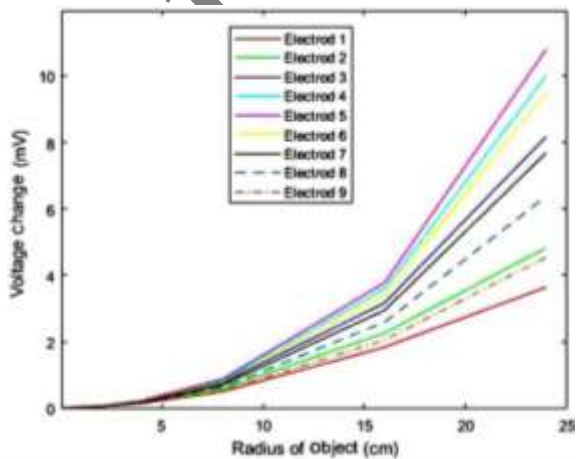
Figure 9 Voltage disturbance of each electrode as a function of the object size.
