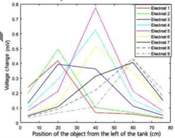
Figure 5 Voltage disturbance of each electrode as a function of the object position.
