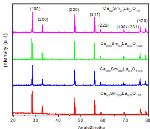
Figure 1. XRD patterns of LSCD- samples
