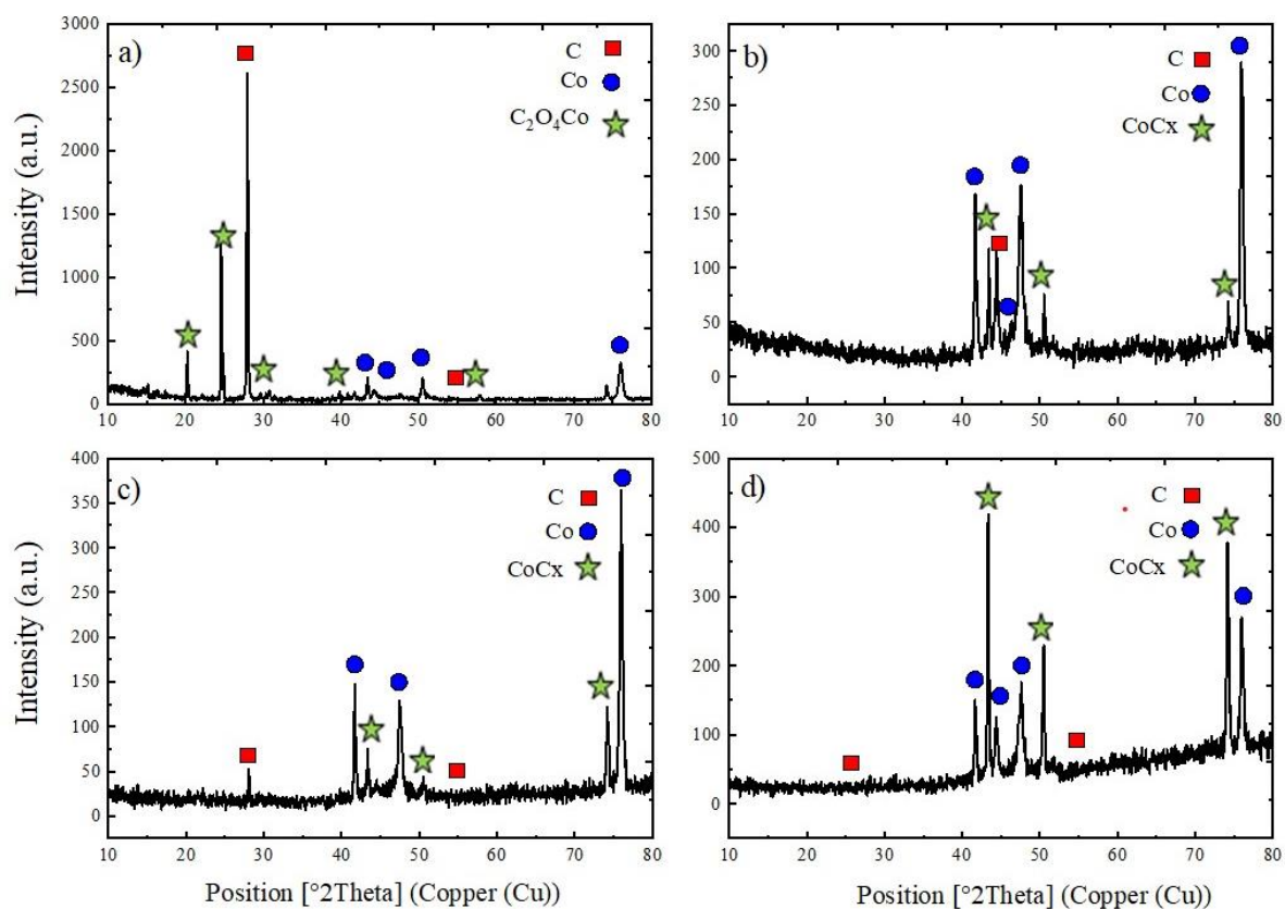
Fig. 5. XRD analysis of samples irradiated by the He plasma jet at different treatment times: (a) 0 s, (b) 30 s, (c) 60 s, and (d) 100 s.
