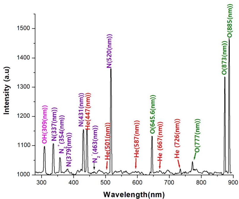
Fig. 4. Spectrum produced by the He plasma jet.
