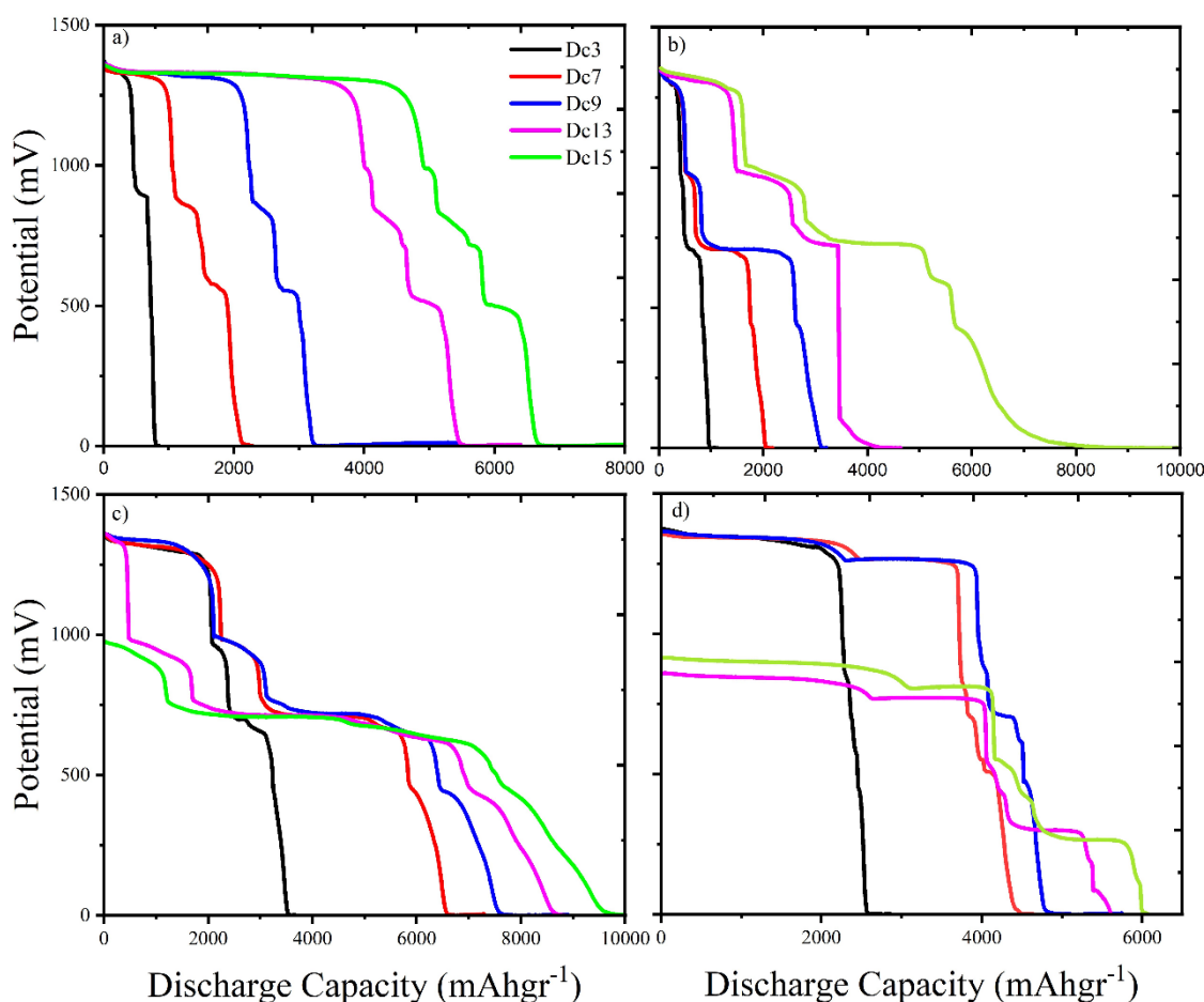
Fig. 7. The hydrogen discharge capacity curves of the Co/MWCNT nanoelectrodes irradiated by He plasma jet at different treatment times (a) 0s, (b) 30s, (c) 60s, and (d) 100s.
