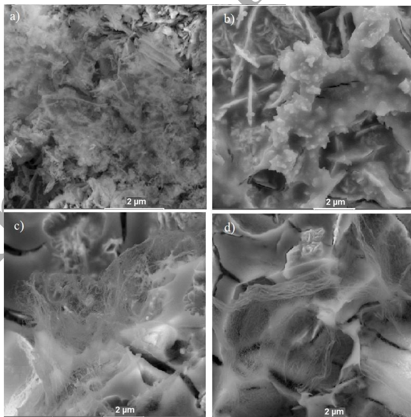
Fig. 6. SEM image of analysis of irradiated Co/MWCNTs composite by He plasma jet at different treatment times (a) 0s, (b) 30s, (c) 60s, and (d) 100s.
