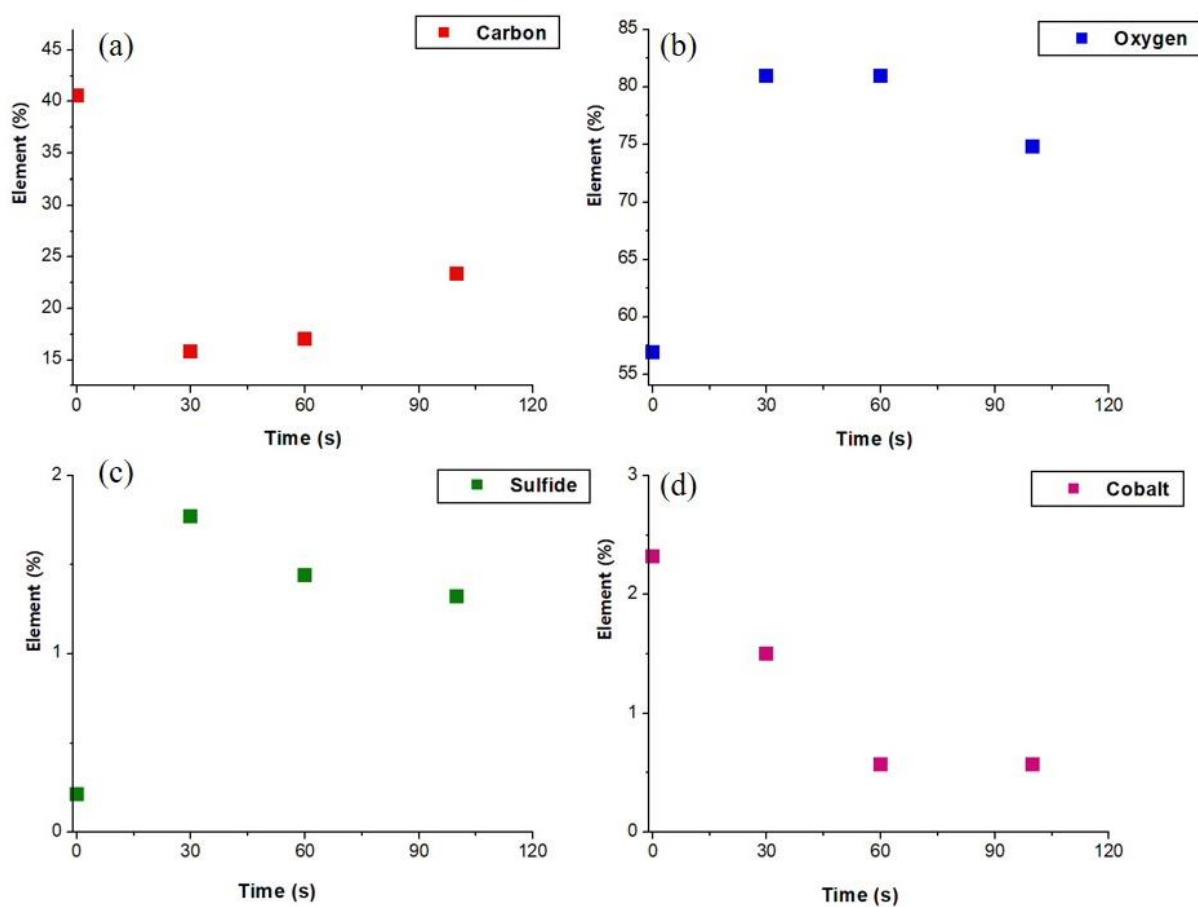
Fig. 3. (a-d) Percentage of different elements (%) versus plasma radiation time.
