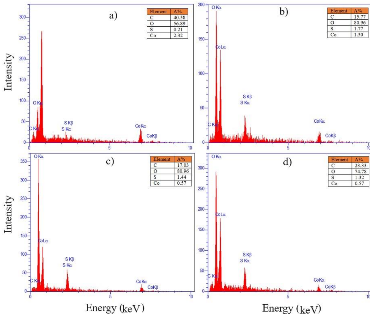
Fig. 2. EDX analysis of Co/MWCNT nanoelectrodes under plasma radiation for (a) 0s (b) 30s, (c) 60s, (d) 100s.
