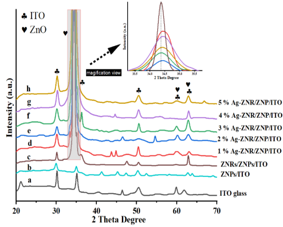
Fig. (3) XRD diffractograms of (a) ITO glass; (b) ZNPs/ITO; (c) pure ZNRs/ZNPs/ITO; and ZNRs doped with different concentrations of Ag: (d) 1%; (e) 2%; (f) 3%; (g) 4%; and (h) 5%.
