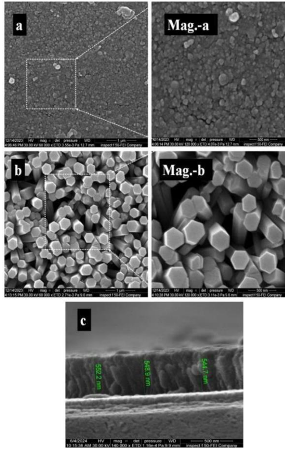
Fig. (4) Field emission scanning electron microscopic images of the (a) ZNPs and (b) ZNRs at different scales and Magnifications; (c) cross-section of pure ZNRs
