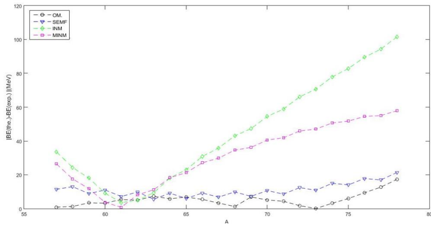
Figure 5. \Delta BE(\text{MeV}) Values calculated using our model for Tin isotopes ^{57-78}_{28}\text{Ni} (in black circle), SEMF (in blue inverse triangle), INM (in green diamond), and MINM (in pink square ).
