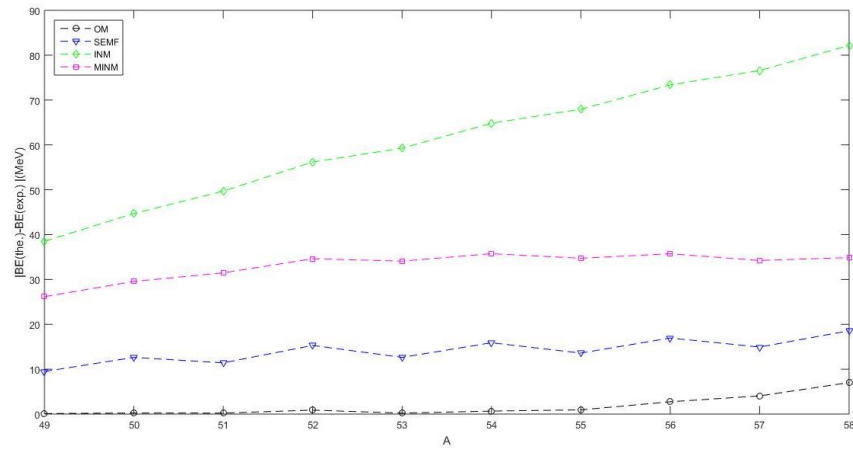
Figure 4. \Delta BE(\text{MeV}) Values calculated using our model for Tin isotopes ^{49-58}_{20}\text{Ca} (in black circle), SEMF (in blue inverse triangle), INM (in green diamond), and MINM (in pink square ).
