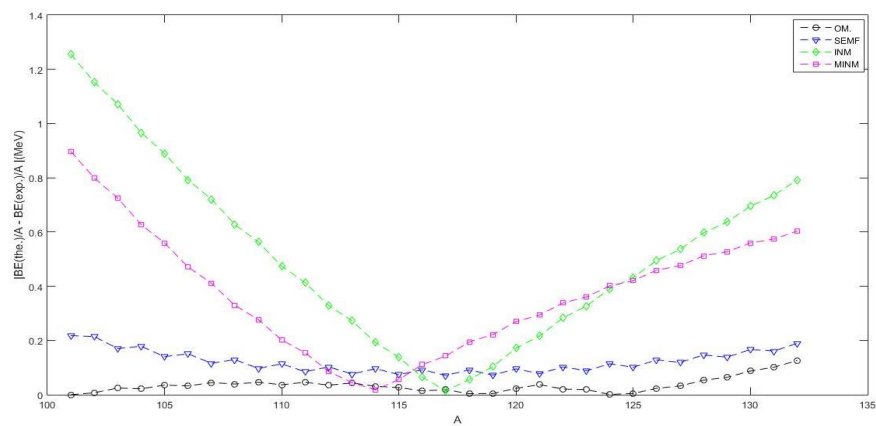
Figure 6. \Delta BE(\text{MeV}) Values calculated using our model for Tin isotopes ^{101-132}_{50}\text{Sn} (in black circle), SEMF (in blue inverse triangle), INM (in green diamond), and MINM (in pink square ).
