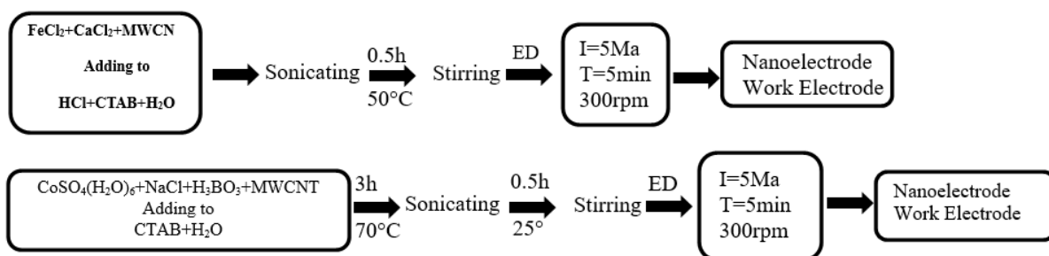
Fig. 1. Schematic flow chart of bath composition and electrodeposition condition.
