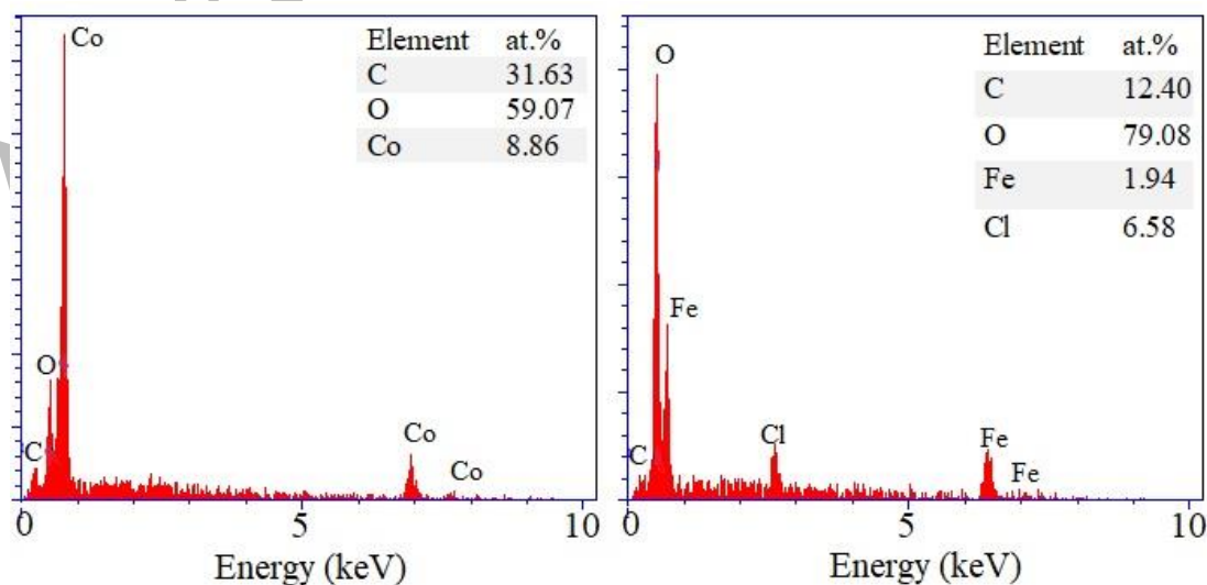
Fig. 3. The EDX spectrum of (a) Co/MWCNT and (b) Fe/MWCNT nanoelectrodes.
