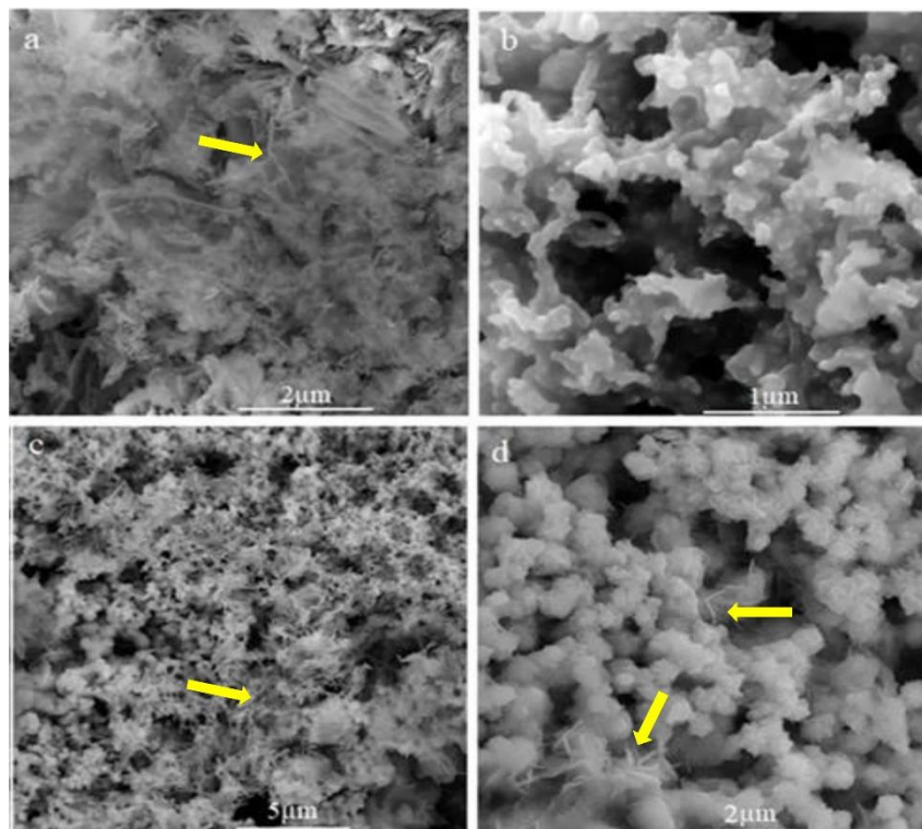
Fig. 4. SEM photograph of (a, b) Co/MWCNT and (c, d) Fe/MWCNT nanoelectrodes.
