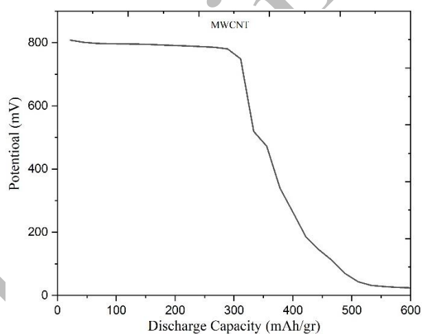
Fig. 5. The first cycle discharge capacity of MWCNTS.
