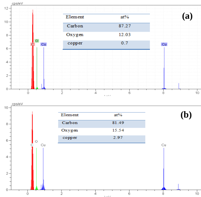
Figure 7. EDX patterns of fCNTs decorated with (a) 2% and (b) 4% of Cu nanoparticles.
