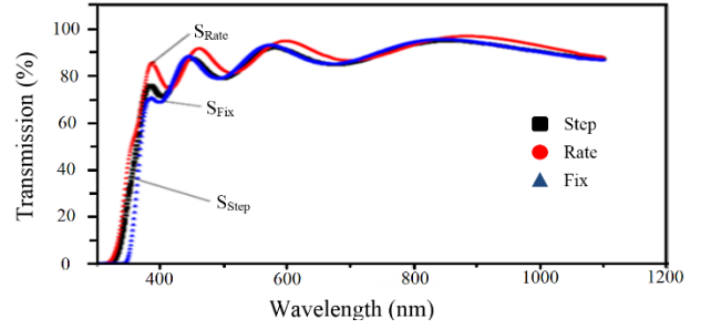
Fig.1. Measured transmission spectra of the deposited \text{TiO}_2 samples at different TTGA process.
