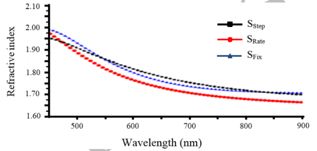
Fig.2. Calculated refractive index of the deposited \text{TiO}_2 thin films at different TTGA process.
