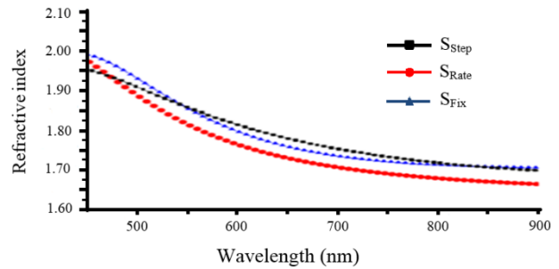
Figure 2. Calculated refractive index of the deposited \text{TiO}_2 thin films at different TTGA process.
