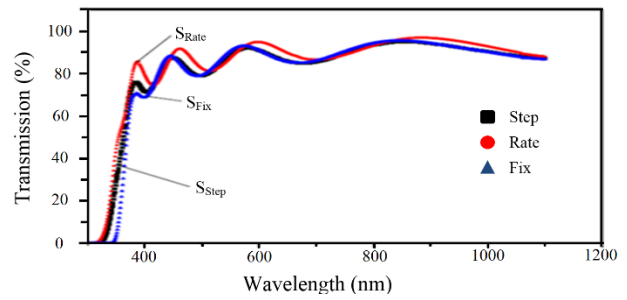
Figure 1. Measured transmission spectra of the deposited \text{TiO}_2 samples at different TTGA process.
