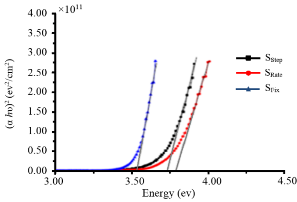
Figure 3. Variation of (\alpha hv)^2 as function of photon energy ( vh )
