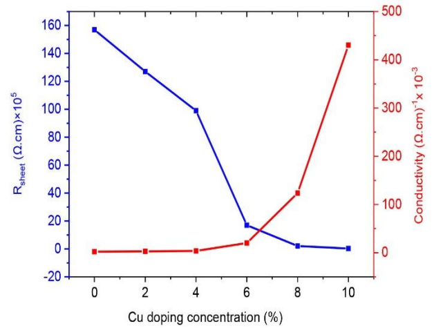
Figure 6. Showcases the variation of the sheet resistance and electrical conductivity of Co 3 O 4 with different concentrations of Cu-doping.
