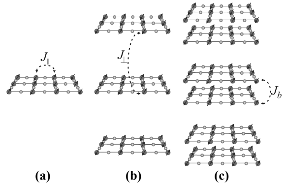
Figure 2. Schematic demonstration of (a) simple square AF case, (b) magnetic structure of LCO4, and (c) magnetic structure of bilayer YBCO6+x.
