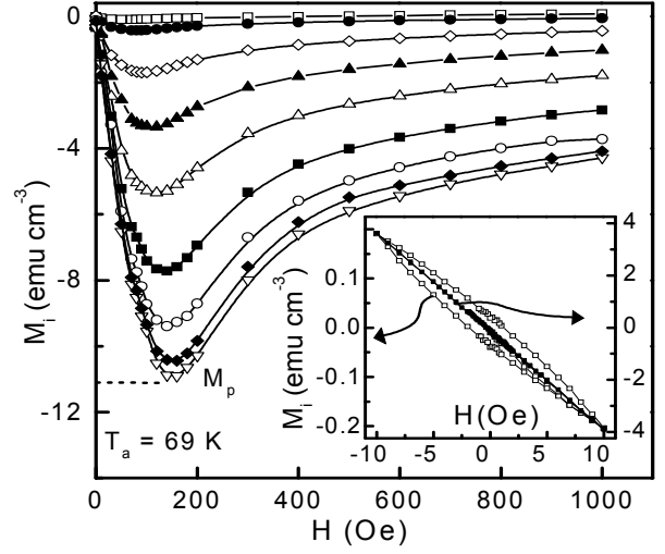
Figure 13. Magnetization M_i vs. H , measured at 2 K, after the same heat treatment (and same symbols) as in figure 12. The peak magnetization is denoted M_p . The solid lines are guides to the eyes. The inset is an expansion of M_i near H = 0 for t_a \approx 0 (left scale) and t_a = 7260 min (right). Note the difference of 18 in the vertical scales.
