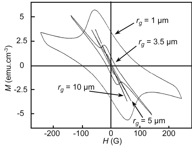
Figure 10. Low field hysteresis cycles for 4 different grain sizes (1 to 10 \mu m). These tiny cycles are typical of ceramic HTS and are signatures of Josephson junctions. The initial slopes are roughly the same for the four samples, but after the suppression of the junctions by the applied field, the slope then decreases with r .
