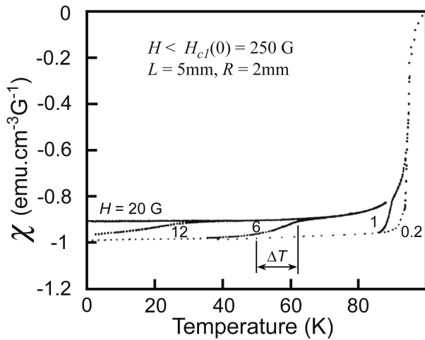
Figure 9. This graph displays the magnetic susceptibility of a sintered YBCO as a function of temperature at different fixed fields. The grains size is of order 10 \mu m. One clearly see the coherent limit and the incoherent-granular limits defined by two envelopes. The steps correspond to the passage from the coherent to the incoherent behavior.
