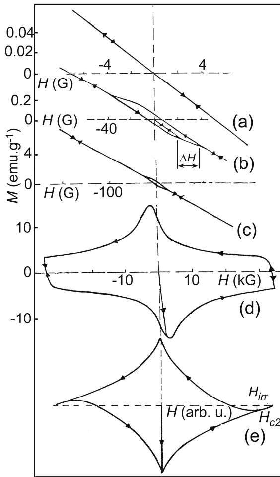
Figure 11. Examples of magnetization loops of sintered granular superconductors at increasing field scales (a, b, c, d) extending from H < H_{c1}^w to H > H_{irr} . Here H_{c1}^w and H_{irr} are the weak link (or Josephson) first critical field and the irreversibility field, respectively (e) Schematic variation of M in the depinning line region. This example is typical of the ceramic \text{YBa}_2\text{Cu}_3\text{O}_7 . At very low H , M is linear, reversible, and exhibits perfect screening if R \gg \lambda_{nl} (the Josephson penetration depth in the weak links). As we will discuss it later this behavior should be common for organic superconductors, however it should be very difficult to observe here, because the Josephson fields and currents as well as the transition temperature are much lower and, more fundamentally, much more distributed in these materials.
