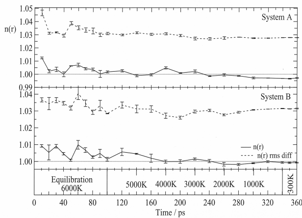
Figure 6. Variation of the spherical average and the absolute deviation of the spherical average from homogeneity for the total spherical average, n(r) , versus time. Simulation temperatures are also indicated. The \pm 1 SD error bars represent the structural variations due to vibrational and translation ionic motion.
