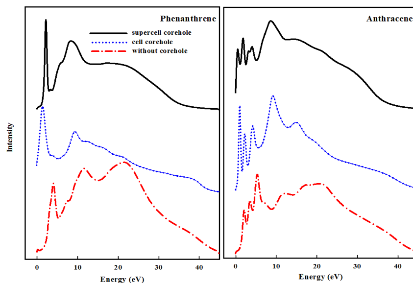
Figure 3. (color online) Super-cell size convergence of the calculated C K edge ELNES spectra of crystalline phenanthrene (left) and anthracene (right).
