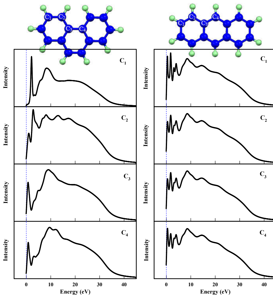
Figure 7. (color online) C K edges ELNES spectra in crystalline phenanthrene (left) and anthracene (right) for the four different carbon atoms represented in the top most figures.
