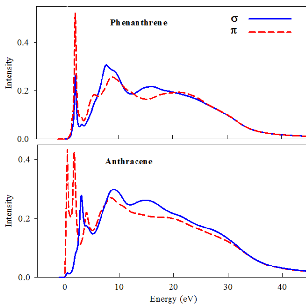
Figure 6. (color online) Spectral ( I' , m' ) decomposition of the ELNES spectra of crystalline phenanthrene (top) and anthracene (bottom). Total spectra are decomposed into the \pi^* (dashed lines) and \sigma^* (full lines) components. As a signature of \pi - \sigma hybridization in both structures, the \sigma^* component overlaps with the \pi^* spectrum at some energy position.
