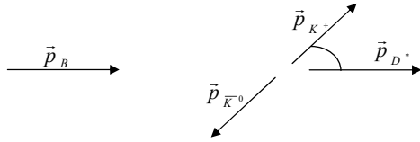
Figure 2. Definition of helicity angle \theta , for the decay.
