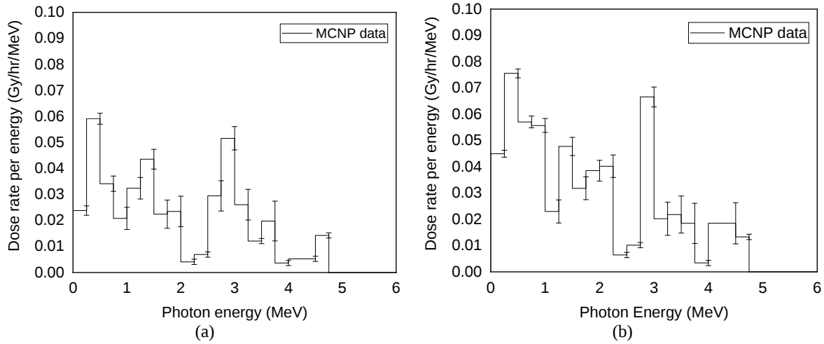
Figure 4. Dose energy spectrum of 6 MeV photon beam at (a) 20 cm and (b) 10 cm depth of water phantom for NE2571 Farmer Chamber.
