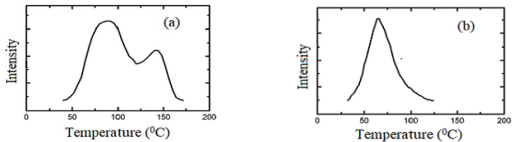
Figure 2. TL spectra for (a) undoped KCl (b) Mn^{2+} doped KCl.
