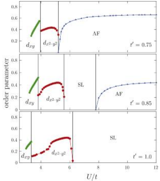
Figure 7. (color online) Same as Figure 6, this time for 2 \times 4 clusters.
