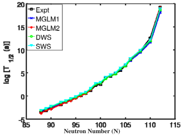
Figure 1. Plots of the calculated \alpha -decay half-lives of Pt isotopes between the various models and experiment.
