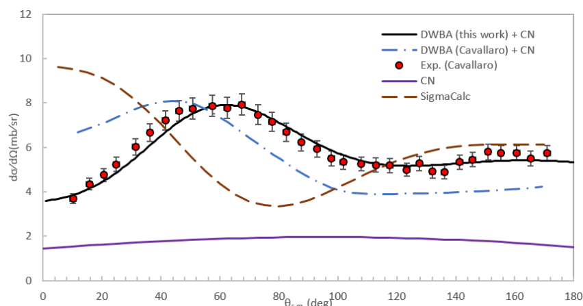
Fig. 4. The angular distribution of ^{16}\text{O}(d,p_0)^{17}\text{O} at 1.6 MeV for the present work along with experimental and theoretical results from the Ref. [7], compound-nuclear (CN) contribution, and the calculation of Ref. [12].
