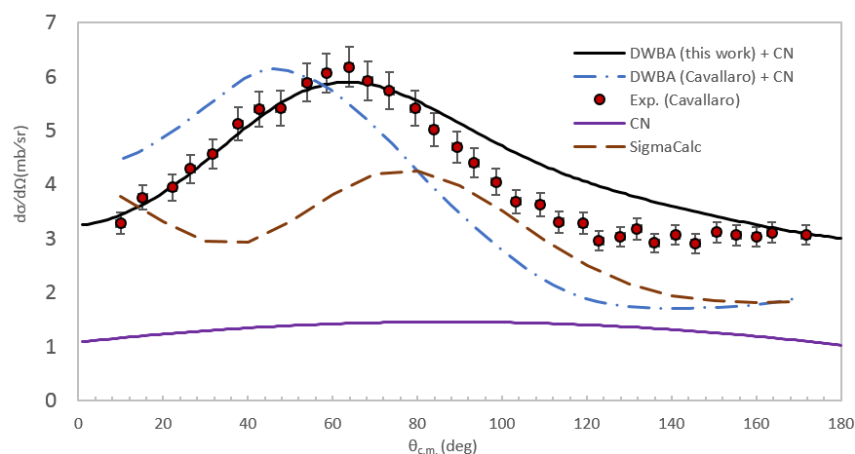
Fig. 3. The angular distribution of ^{16}\text{O}(d,p_0)^{17}\text{O} at 1.3 MeV for the present work along with experimental and theoretical results from the Ref. [7], compound-nuclear (CN) contribution, and the calculation of Ref. [12].
