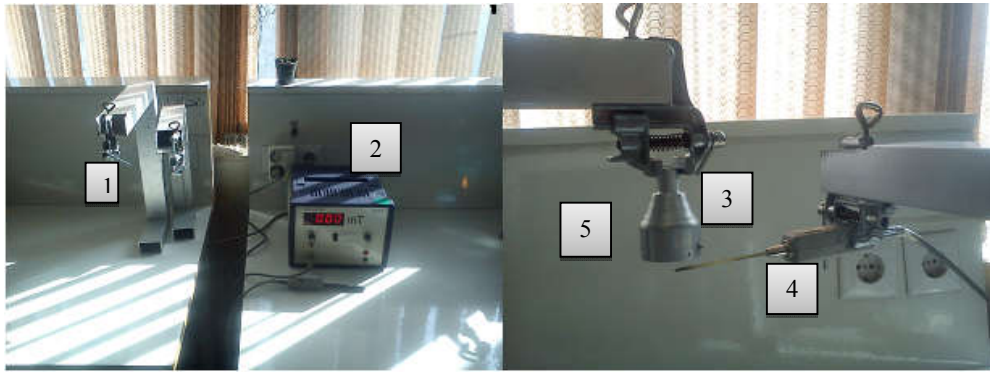
Figure 9. (color onlin) Measurement equipment (1) Aluminum stands, (2) phvwe teslameter device with a probe, (3) aluminum hook, (4) measurement probe, and (5) magnet aluminum fixture.
