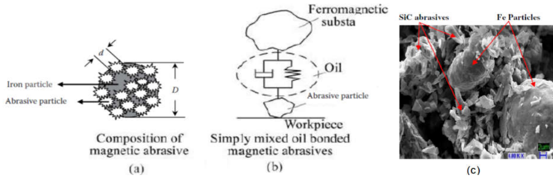
Figure 3. (color onlin) Schematic of (a) bonded, (b) unbonded magnetic abrasive particles, and (c) SEM micrograph of unbounded SiC abrasives (800 mesh).
