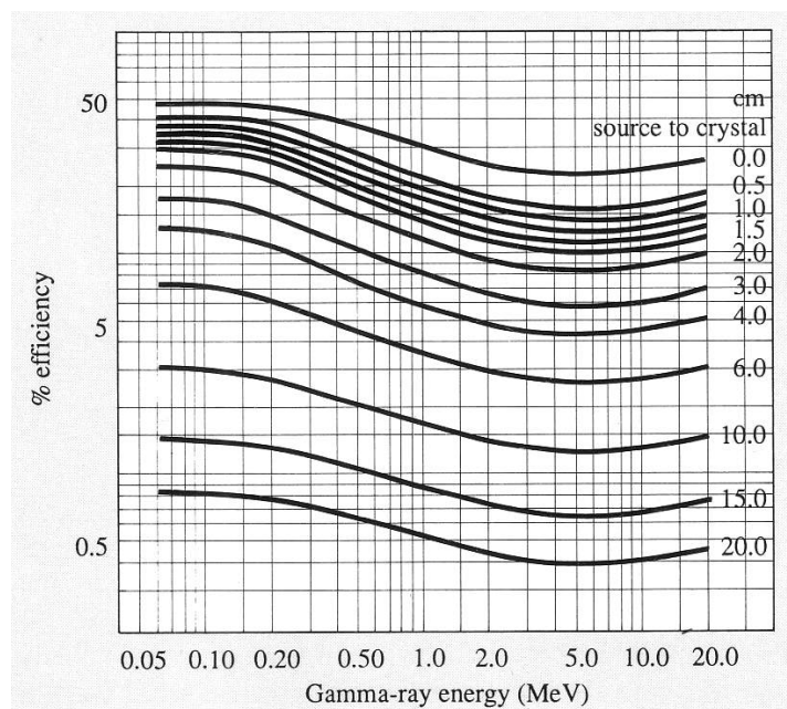
Figure 2. Calculated efficiencies for a typical scintillation detector as a function of the gamma-ray energy and source to detector distance.
