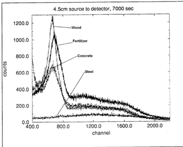
Figure 5. The spectra of four materials.
