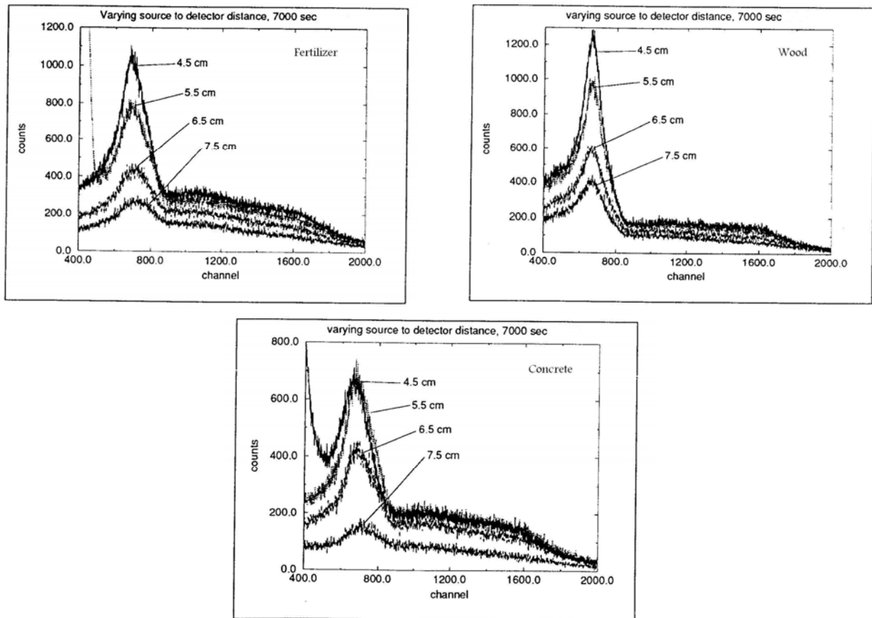
Figure 4. Compton scatter spectra for three materials.
