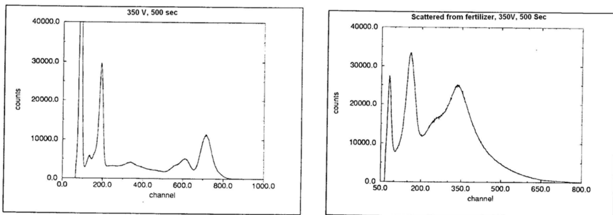
Figure 3. Barium spectrum before and after using organic fertilizer.
