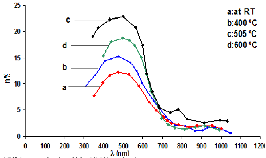
Figure 5. (color online) Efficiency as a function of \lambda for CdS/Si heterojunction.
