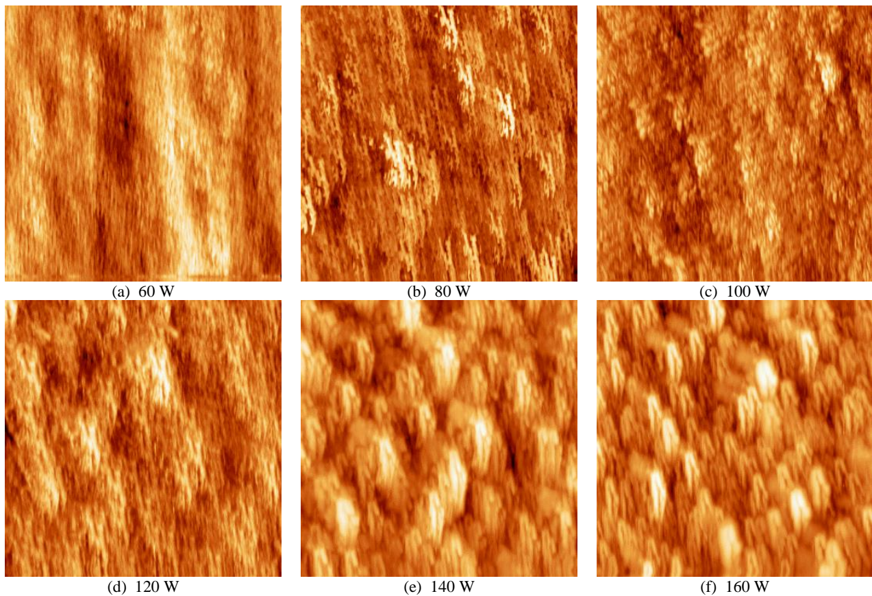
Figure 6. AFM Surface morphology ( 3 \times 3 \mu\text{m} ) of Zr films deposited on Si substrate at different power (from 60 to 160 W).
