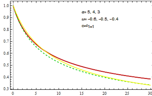
Figure 2. Graph of energy density parameter \rho(t) versus cosmic time t .
