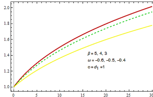
Figure 5. Graph of scale factor parameter a(t) versus cosmic time t .
