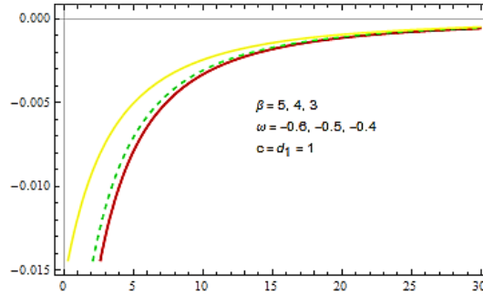
Figure 7. Graph of cosmological constant parameter \Lambda(t) versus time t .
