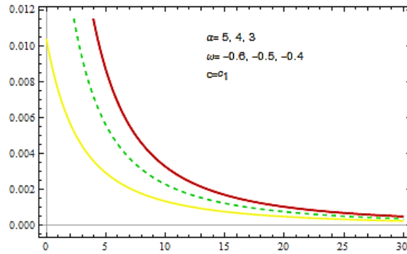
Figure 3. Graph of DE model parameter \Lambda(t) versus cosmic time t .
