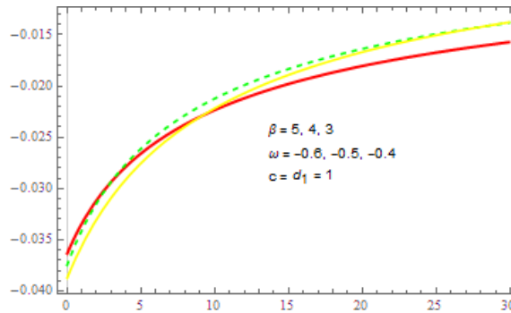
Figure 8. The evolution of time dependent gravitational constant parameter G(t) versus cosmic time ( t ).
