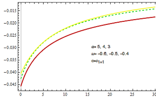
Figure 4. Graph of time dependent gravitational constant parameter G(t) versus cosmic time (t) .
