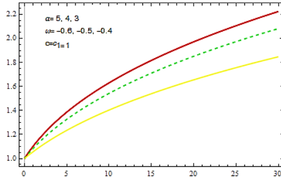
Figure 1. The graph of scale factor parameter a(t) versus cosmic time (t) .
