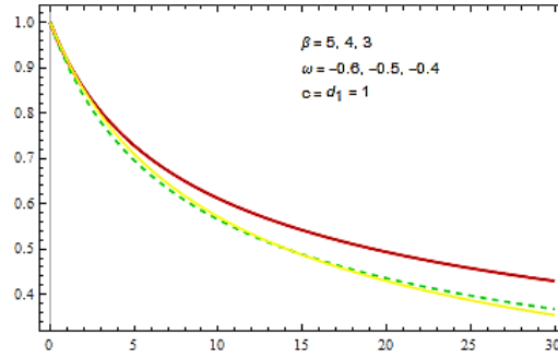
Figure 6. Graph of energy density parameter \rho(t) versus cosmic time t .
