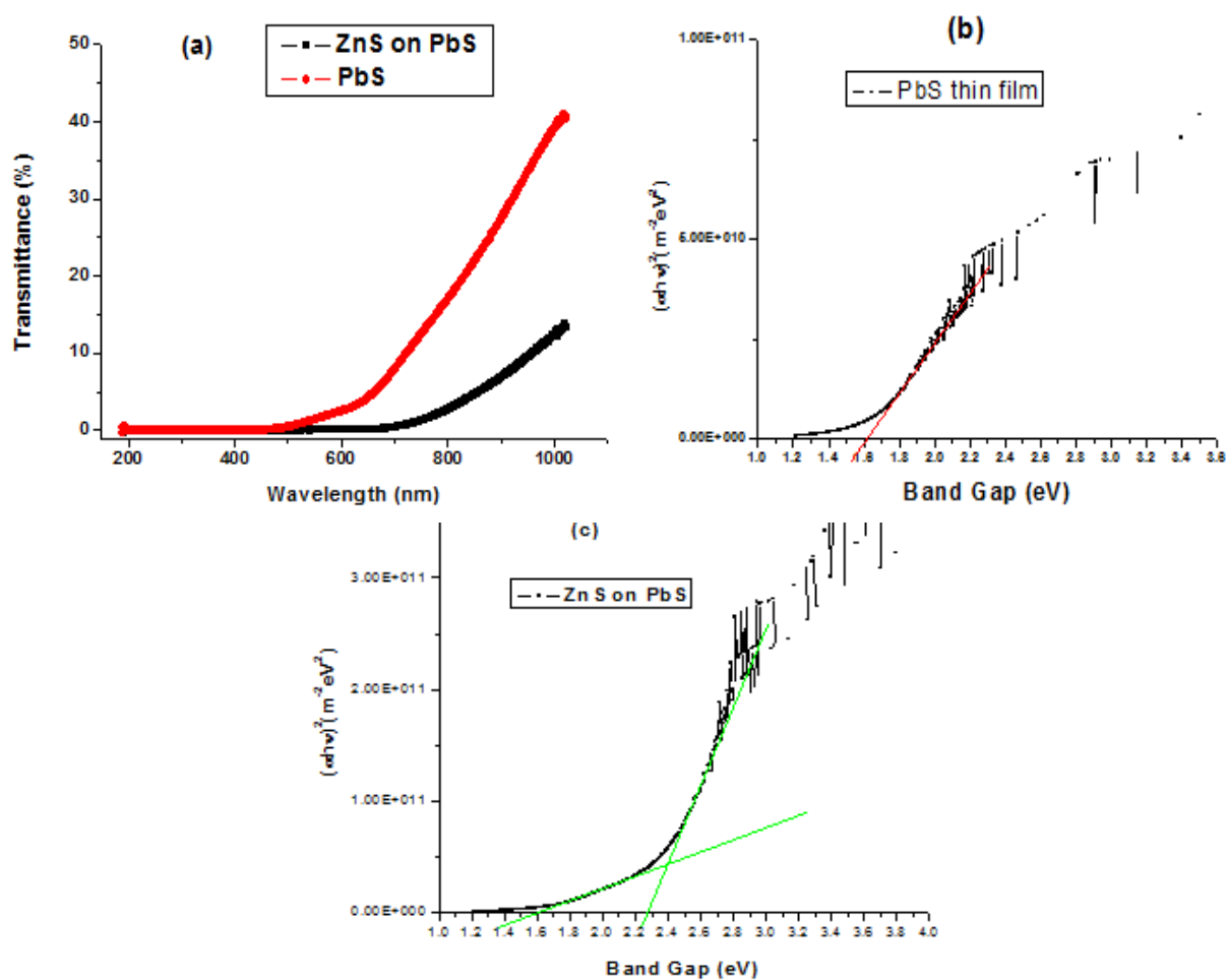
Figure. 7 (a) UV-Vis spectra for PbS (red color) film and ZnS/PbS nanowires (black color) and their corresponding band gap (b) for PbS thin film and (c) ZnS/PbS nanowires deposited on glass substrates.
