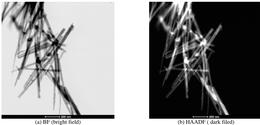
Figures. 4 HRTEM images (a) BF (bright field) and (b) HAADF (dark filed) mode.
