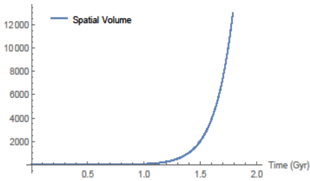
Figure 1. Depicts this behavior of volume V versus time t . Also, when t \rightarrow \infty , scale factors a, b, c and D are found to be infinite.
