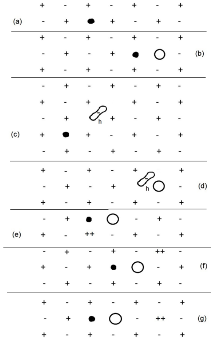
Figure 1. Arrangement of ions in a NaCl lattice: Alkali ions are shown as + and chloride ions as -. The electron occupying anion vacancy is shown by a thick dot. The vacant sites are indicated by circles. The letter h represents a hole in \text{Cl}_2^- . Possible defects are indicated by markers (a), (b), (c), (d), (e), (f) and (g) viz. (a) Secluded F-center, (b) bi-vacancy, (c) V_k -center linked to anion vacancy, (d) V_F center, (e) Linked divalent cation, (f) nn I-V pair linked to anion vacancy and (g) nnn I-V pair linked to anion vacancy.
