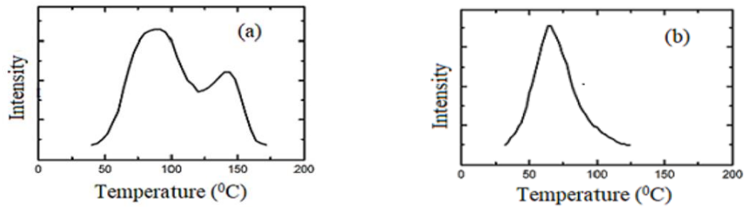
Figure 2. TL spectra for (a) undoped KCl (b) \text{Mn}^{2+} doped KCl.
